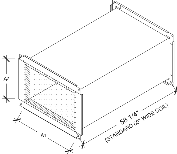
DOUBLE WALL COIL-LINE DUCT
