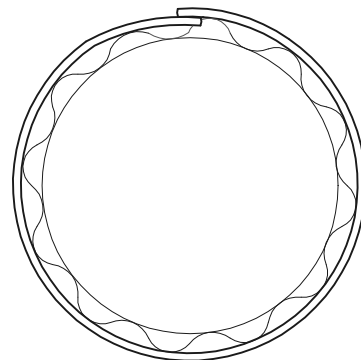
LAPPED, TACKED (OR SPOT WELDED) & SEALED
