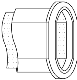
ACCUFLANGE (DOUBLE WALL) * = 1"DW, 2"DW OR 3" DW
