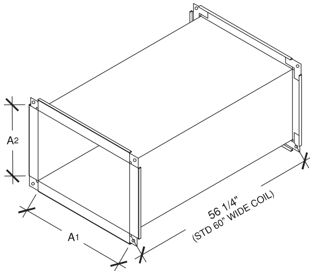
COIL-LINE DUCT TDC CONNECTION
